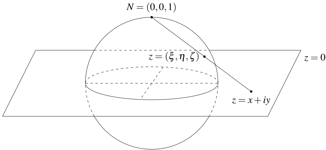
Figure 3.1: Stereographic projection
